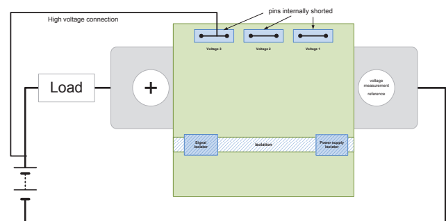
Figure 7: example for voltage measurement
