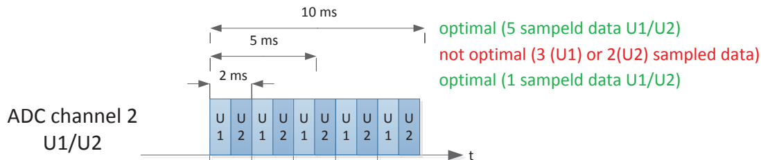
Figure 13: example with two channel on ADC2
